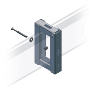
Wall Installation
